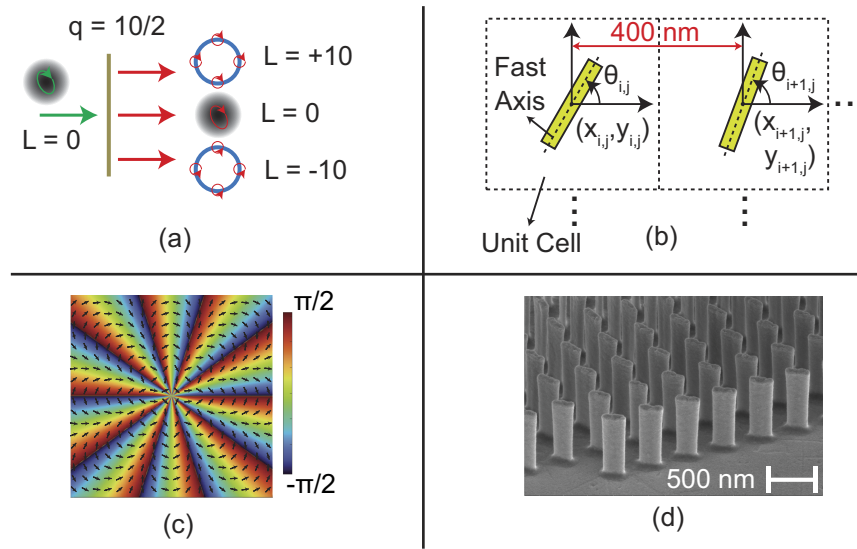
Fig. 2. Tunable excitation of l = \pm 10 modes using a metasurface q-plate. (a) Schematic of a q-plate of order q = |l|/2 = 10/2 . For an input Gaussian beam for some elliptical state of polarization, the output consists of a mixture of the l = \pm 10 free-space OAM beams as well as an unconverted Gaussian remnant. (b) Illustration showing a unit-cell of the metasurface q-plate, consisting of an amorphous Si nanofin that acts as a half-wave plate, with fast-axis orientation \theta_{i,j} and spatial position (x_{i,j}, y_{i,j}) on the spatial grid. The separation between adjacent unit cells is 400 nm. (c) Colormap overlaid with a quiver plot showing the 2-dimensional spatial distribution of unit cell fast axes orientations on the metasurface. The orientation of the fast axes is given by \Theta = |l|\phi for |l| = 10 , where \phi is the angular coordinate. (d) Scanning electron micrograph of the fabricated metasurface q-plate showing individual nanofins
