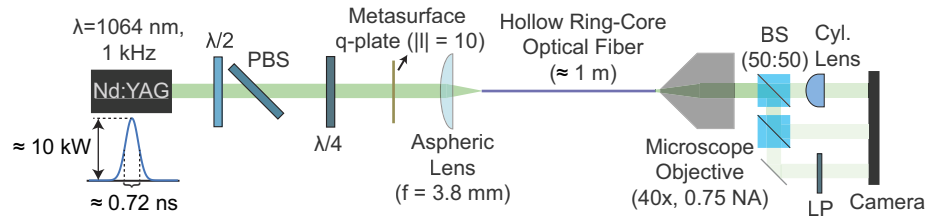
Fig. 3. Schematic of the experimental setup constructed to study nonlinear rotation of spin-orbit coupled states in hollow RCFs.
