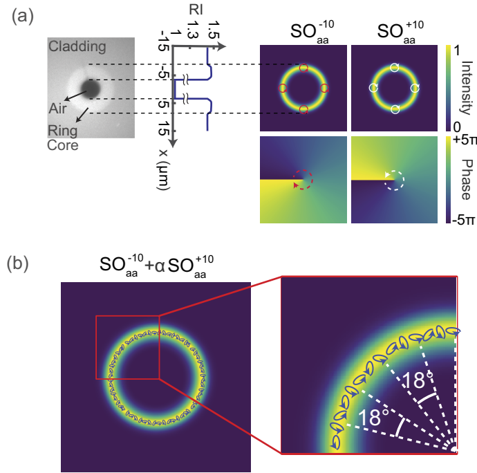
Fig. 1. Modes of a hollow ring-core fiber. (a) Optical micrograph of the cross-section of hollow RCF, overlaid with the refractive index profile. The intensity, polarization and phase profiles of the l = \pm 10 SO_{aa} modes are shown. Note that the modes have opposite helicities of polarization and phase. (b) A superposition of the two modes with \alpha \neq 1 results in a spatially varying elliptical state of polarization. The ellipticity at each point is the same, and is determined by the relative amplitudes, while the orientation of the ellipses rotates 2\pi every 360^\circ/(2|l|) = 18^\circ .
