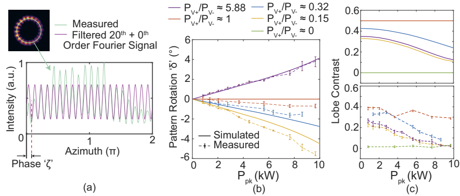
Fig. 6. Fourier analysis of nonlinear rotation via image processing. (a) Illustrative example showing the image processing routine. The intensity pattern along a thin circular ring concentric with the lobe pattern is extracted from the recorded images, and Fourier filtering is performed to retain only the 20 th and 0 th order components. The rotation of the lobes \delta is recovered from the change in Fourier phase \zeta of the azimuthal intensity signal with a change in input peak power. The lobe contrast is defined as the magnitude ratio of the 20 th and 0 th order Fourier components. (b) Rotation \delta of the time-averaged lobe pattern at various input powers, for simulation (solid line plots) and experiment (dotted line plots). The plot also shows the control cases of input SOP being circular and linear. (c) Simulated (top; solid line plots) and experimentally measured (bottom; dotted line plots) reduction in lobe contrast as a function of input power.
