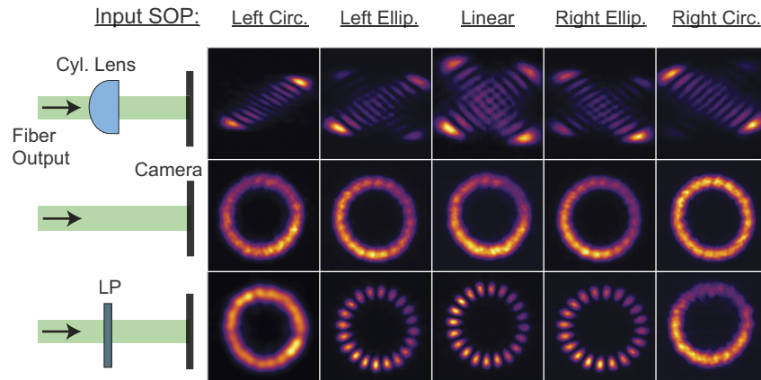
Fig. 4. Demonstration of tunable excitation of l = \pm 10 SO_{aa} modes in a hollow RCF using a metasurface q-plate: experimental images. The beam exiting the fiber is imaged at different input SOPs. (Top) A cylindrical lens is used to convert the LG beam emerging from the fiber to the HG basis, to reveal the OAM mode content in the fiber. (Middle) Polarization-insensitive measurement of the intensity pattern of the output beam. (Bottom) When imaged through a linear polarizer, 2|l| = 20 lobes appear for all input SOPs except for LCP and RCP, each of which excite purely one OAM mode.
