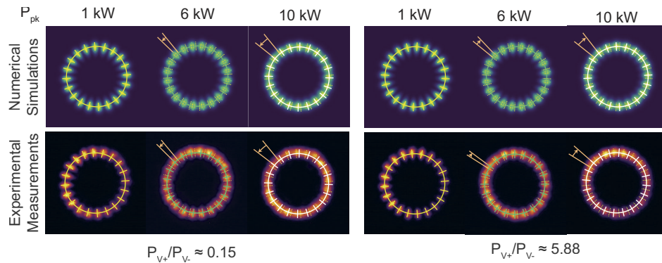
Fig. 5. Nonlinear rotation of unequal superpositions of the l = \pm 10 SO_{aa} modes: numerical simulation and experimental images of the time-averaged output intensity pattern imaged through a linear polarizer, at various input peak powers, for two values of mode power ratios P_{V+}/P_{V-} . For visual aid, a wheel pattern is aligned with the lobes and overlaid on top of the images. Notice that the wheel patterns at the different power levels are not aligned with each other, indicating a power-dependent rotation. Also note the opposite sense of rotation in the dominant l = -10 case vs the dominant l = +10 case.
